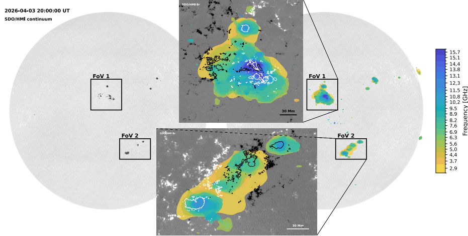
Figure 1: EOVSAs active-region footprints at 2.9–15.7 GHz over HMI continuum and radial-field maps. Their contraction with increasing frequency illustrates how broadband source boundaries sample progressively stronger coronal fields. The colors mark frequency, not intensity. Adapted from Yu et al. (2026).
