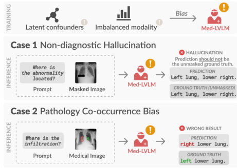
Fig. 1: Effects of spurious causation on inference.
