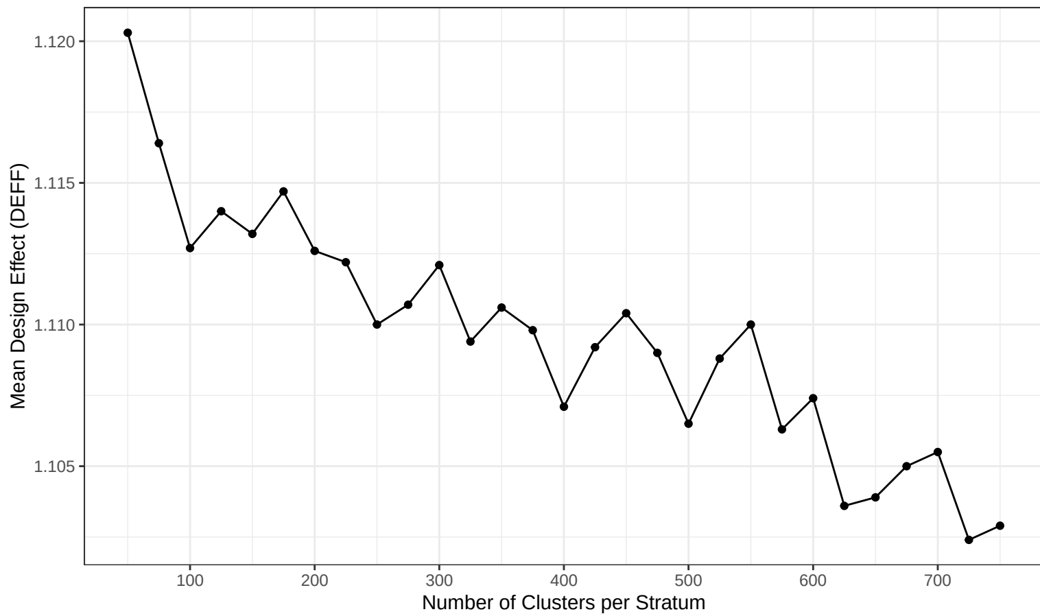
Mean Design Effect by Number of Clusters
