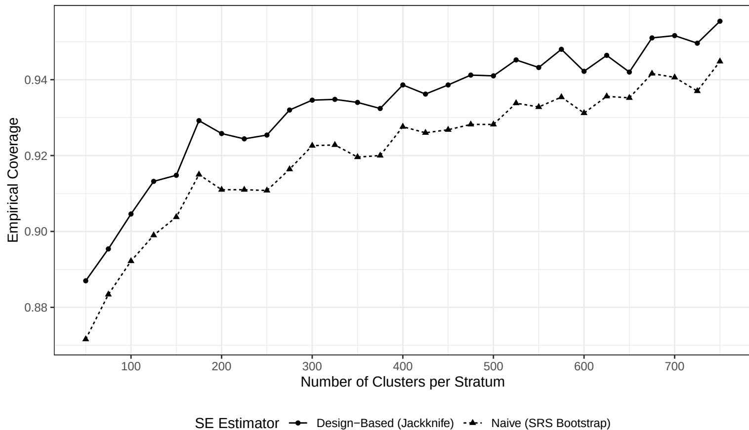
Empirical Coverage by SE Estimator
