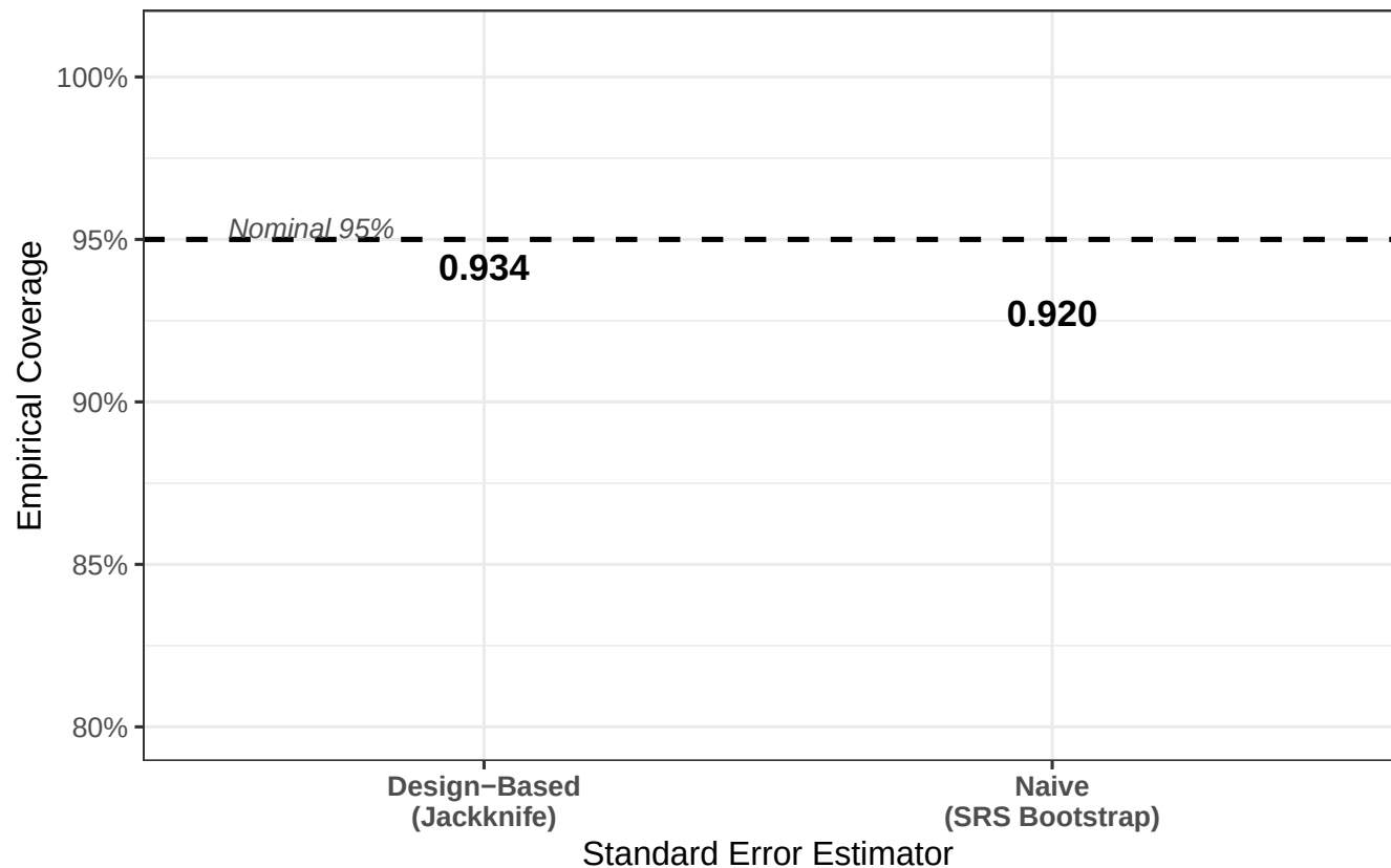
Figure 3 (Objective ii) – Empirical Coverage of 95% Wald Confidence Intervals
