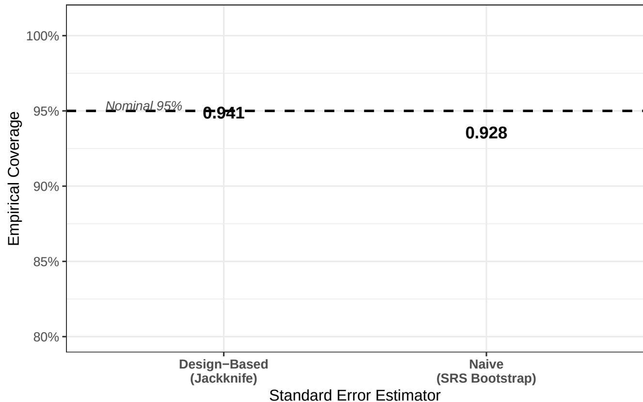
Figure 3 (Objective ii) – Empirical Coverage of 95% Wald Confidence Interval
