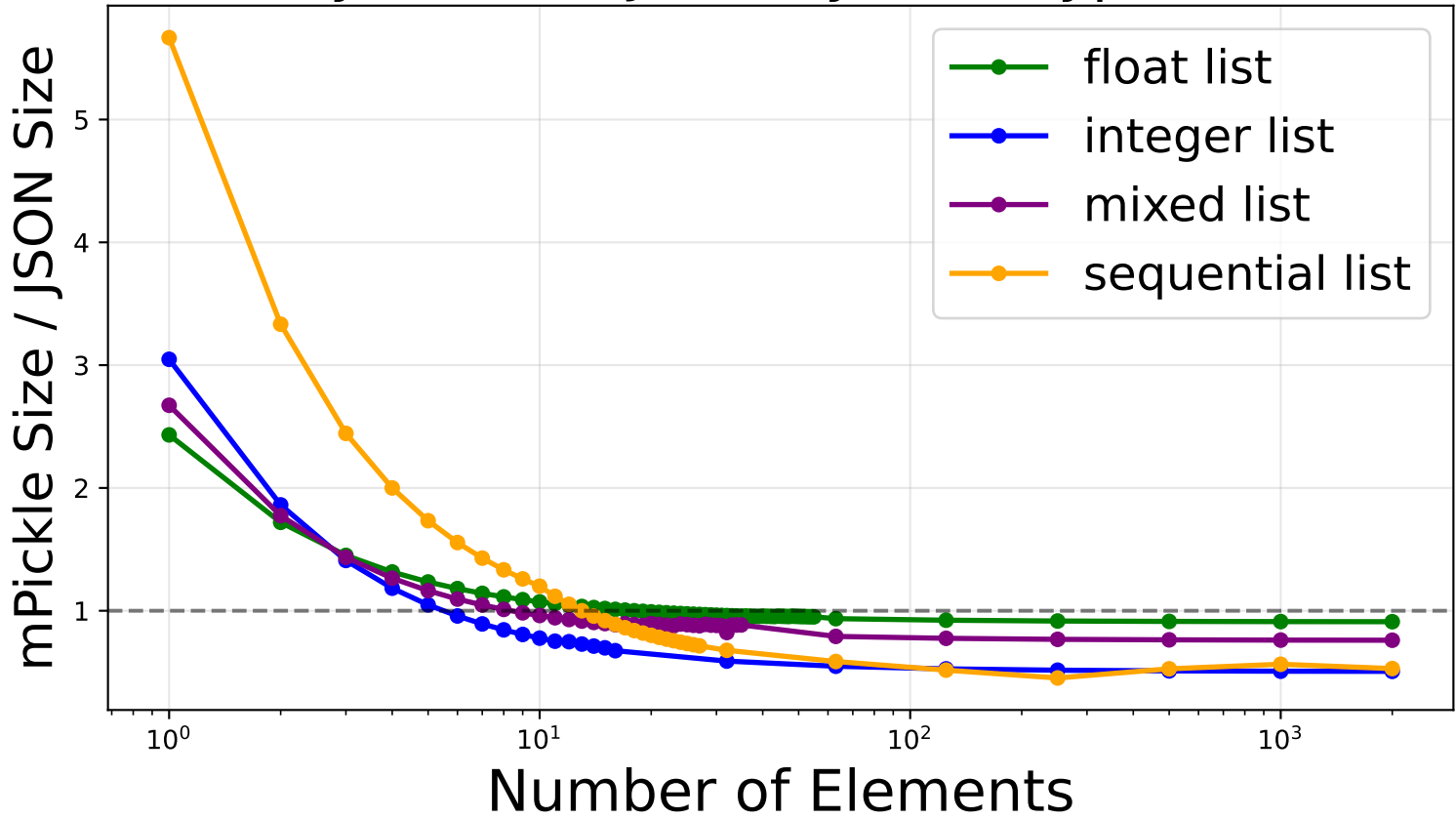
mPickle Efficiency Ratio vs JSON by Data Type (1-2000 elements)
