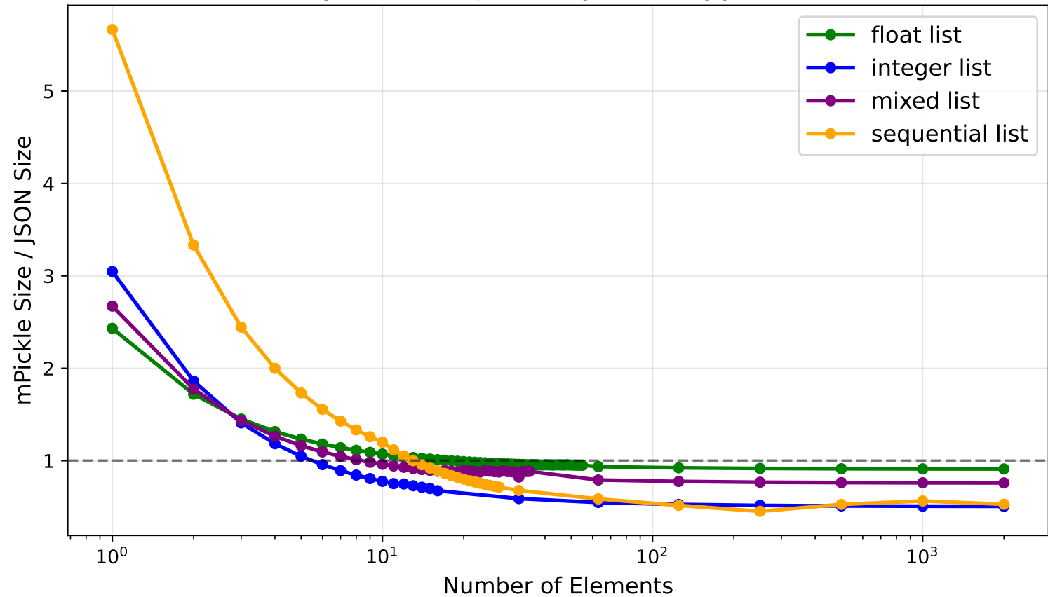
mPickle Efficiency Ratio vs JSON by Data Type (1-2000 elements)
