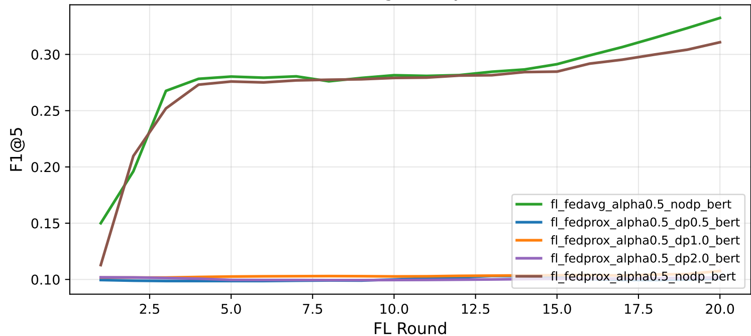
FL Convergence by Round
