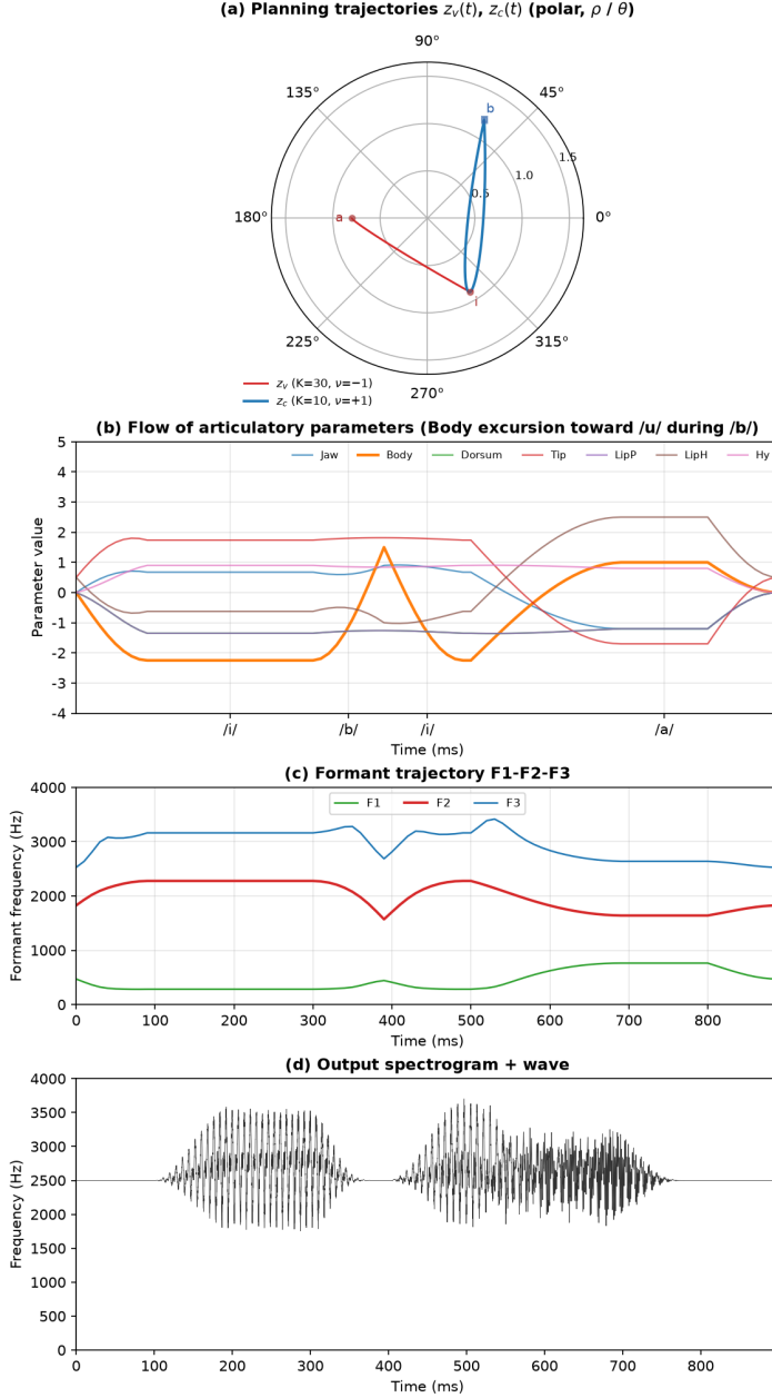
Figure 1: four-step synthesis of /ibia/ — T = 100 ms ( K=10 , K_{voy}=30 , P_{exp}=1 ) arXiv:2307.02299 (Berthommier 2023)
