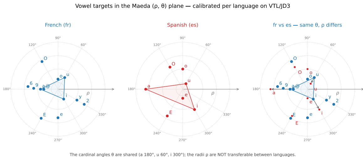
Figure 2: Vowel targets of French (blue) and Spanish (red) in the (\rho, \theta) plane, read directly from the shipped language blocks. Left/middle: each language with its a-i-u triangle. Right: overlay — the cardinal angles are shared, the radii differ (French /i/ \rho = 0.34 vs Spanish /i/ \rho = 0.70 at the same 300^\circ spoke).
