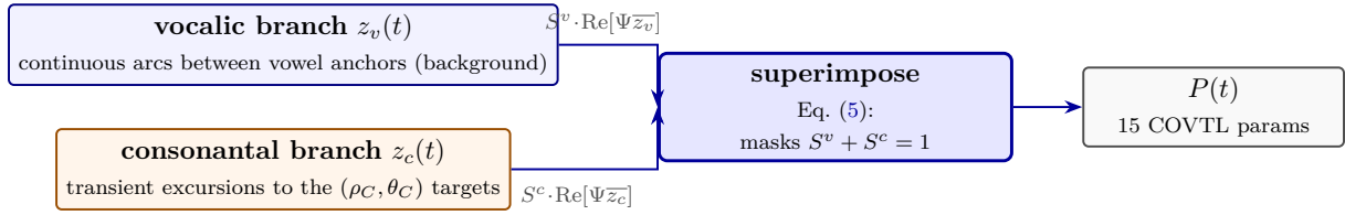
Figure 2: The two-branch superposition of Eq. (5). Each tract parameter belongs to exactly one branch at each instant: the consonant selector decides which.
