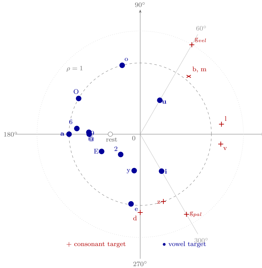
Figure 1: The (\rho, \theta) phonetic plane of the COVTL model, drawn to scale from the target tables of constants.py . Filled dots: the 12 vowel targets (Table 1); crosses: landmark consonant targets (Table 2). The dashed unit circle is the frontier of the vowel space; consonant closures live beyond it ( \rho > 1 ). The schwa @ sits at the centroid of the calibrated a-i-u triangle. /m/ coincides with /b/ — same target and same selector; only the velum extension (VO, outside the COVTL selector) differs.
