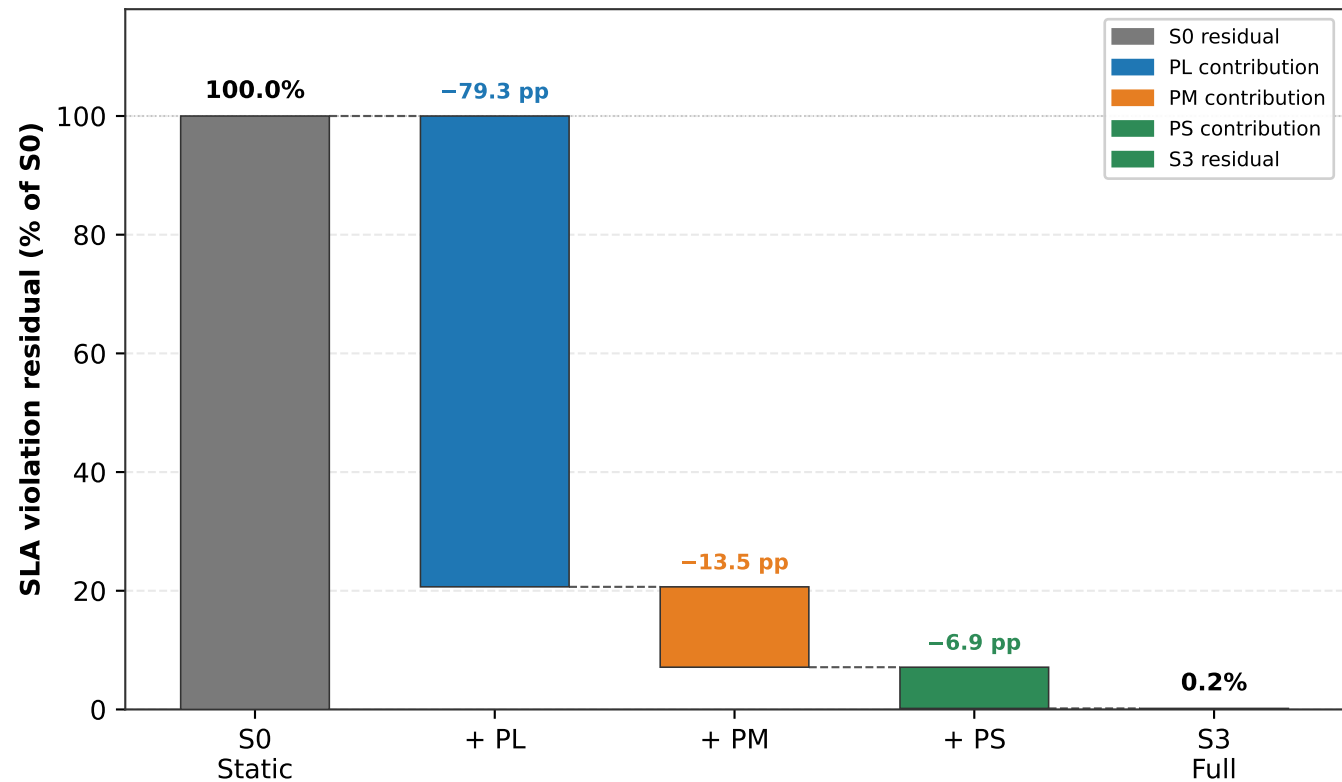
Figure 4A: SLA Violation Reduction (layer waterfall)
