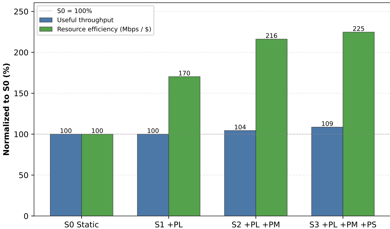
Figure 4C: Throughput and Resource Efficiency
