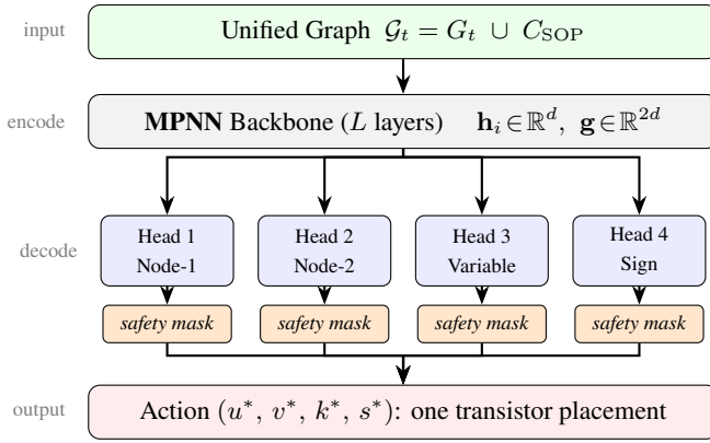
Figure 2: Architecture of the Switching Graph Policy Network (SGPN). The unified graph \mathcal{G}_t = G_t \cup C_{\text{SOP}} is encoded by a shared MPNN backbone; four factored heads with per-head safety masks decode the transistor-placement action (u^*, v^*, k^*, s^*) .
