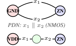
(c) AND2 CMOS dual
