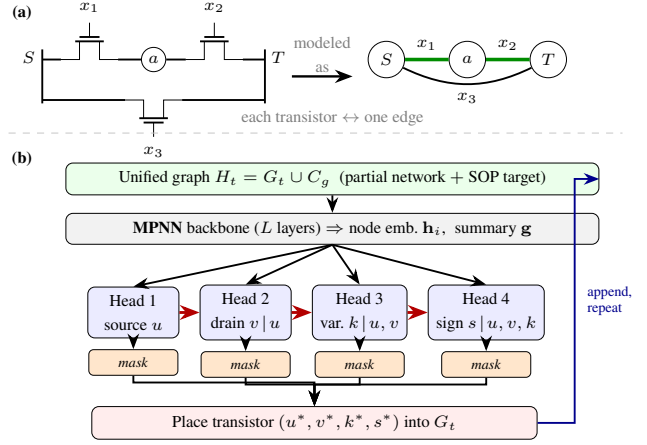
Figure 2: (a) A transistor network is a switching graph: an input pattern yields a conducting source-to-sink ( S \rightarrow T ) path exactly on the on-patterns of the target (coverage), and no path on the off-patterns (safety). (b) The Switching Graph Policy Network (SGPN) synthesizes such a network one transistor at a time. A shared MPNN backbone encodes the unified graph H_t = G_t \cup C_g (the partial network fused with the fixed SOP target); the four heads then fire sequentially —source u , drain v , variable k , sign s —each conditioned on the earlier selections and its own safety mask. The placed transistor (u^*, v^*, k^*, s^*) is appended to G_t and the step repeats until the network covers the target.
