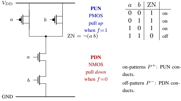
Figure 1: A CMOS standard cell for f = \neg(a b) (NAND2). Each transistor is a literal-controlled switch (Def. 1): the pull-up network (PUN, PMOS in parallel) drives the output ZN high on the on-patterns of f , and the pull-down network (PDN, NMOS in series) drives it low on the off-patterns. Synthesizing the cell therefore splits into two switching-network problems—one per network (Prop. 1).
