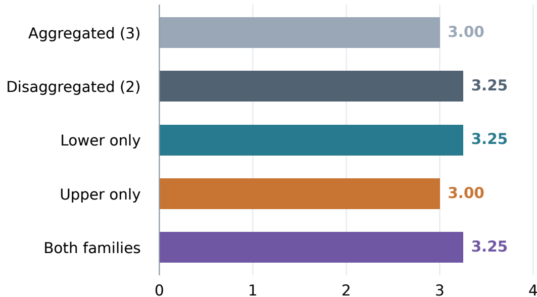
Linear relaxation value
