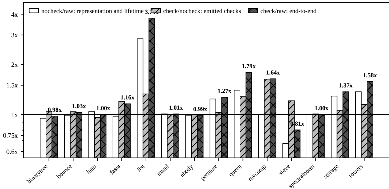
median runtime ratio (log scale)
