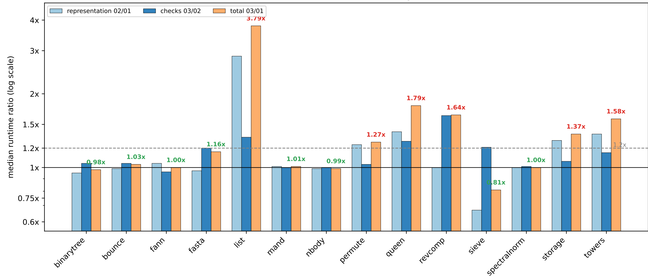
Three-state cost decomposition: representation (02/01), checks (03/02), and total (03/01) 14 benchmarks, total cost \leq 1.2x in 8/14 (green), rest red
