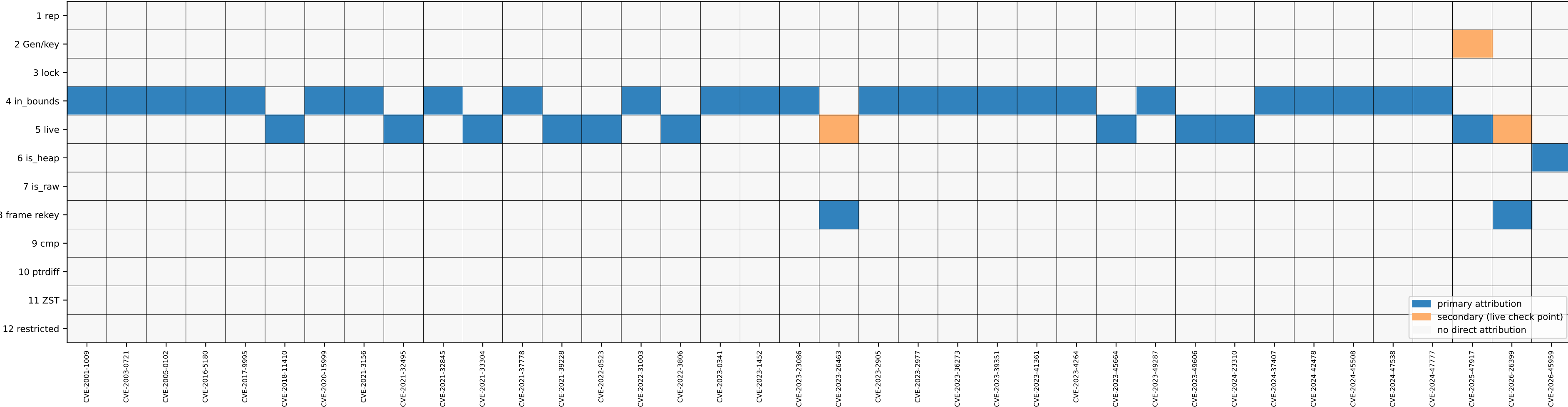
CVE interception matrix: 38 CVEs x 12 mechanisms (tests/fat_cve, MECHANISMS.md backfilled adb102a) attribution: 4 in_bounds 25 . 5 live 10 . 6 is_heap 1 . 8 frame rekey 2 (+2 secondary)
