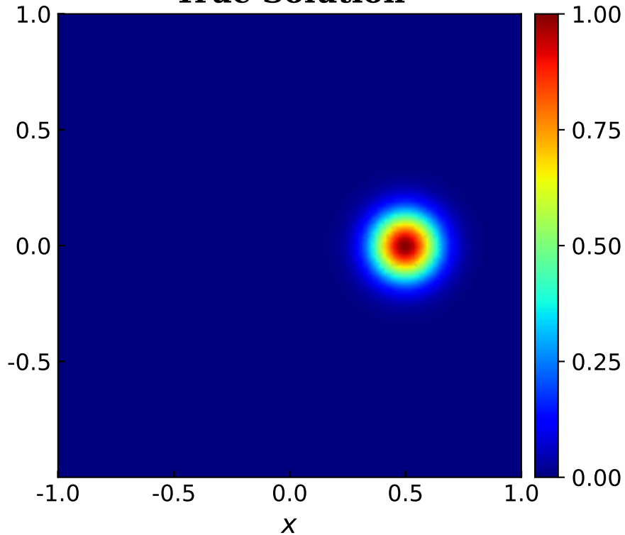
True Solution
