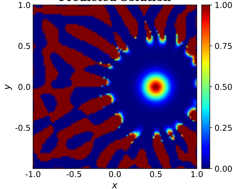
Predicted Solution
