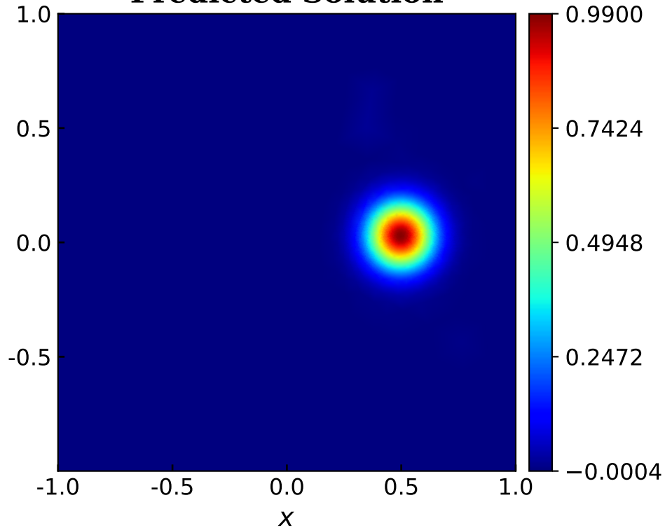
Predicted Solution
