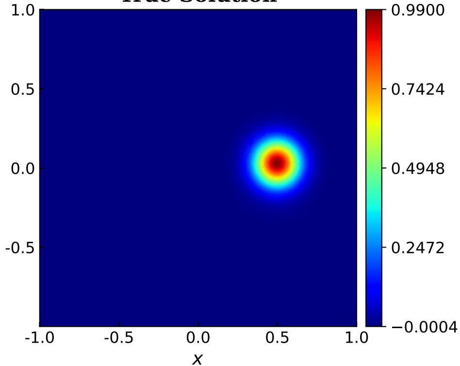
True Solution
