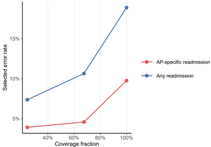
Selective risk after conformal abstention
