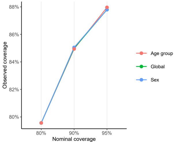
Empirical conformal coverage
