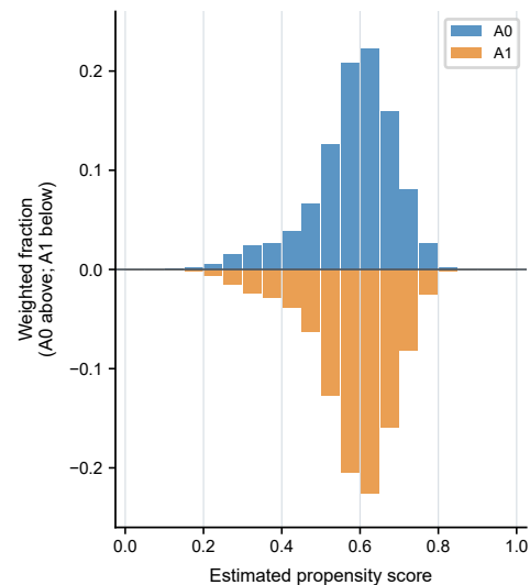
b Aggregate overlap after weighting
