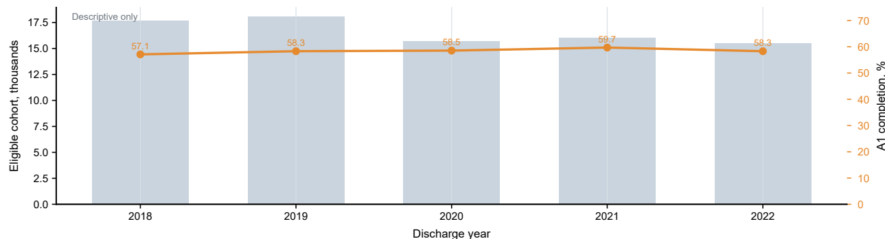
c Annual cohort and completion reporting
