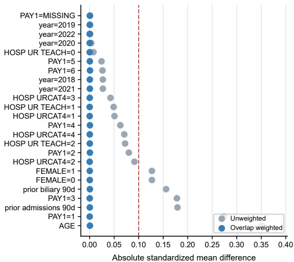
a Selected covariate balance
