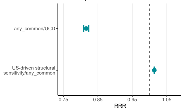
Overall representation RRRs
