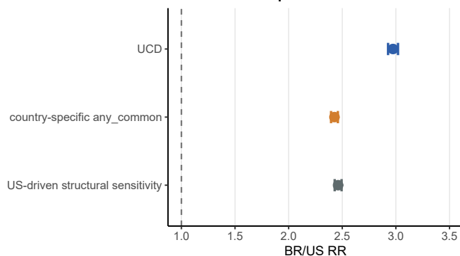
Overall BR/US representation RRs
