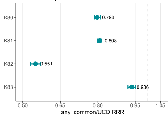
K80-K83 component RRRs
