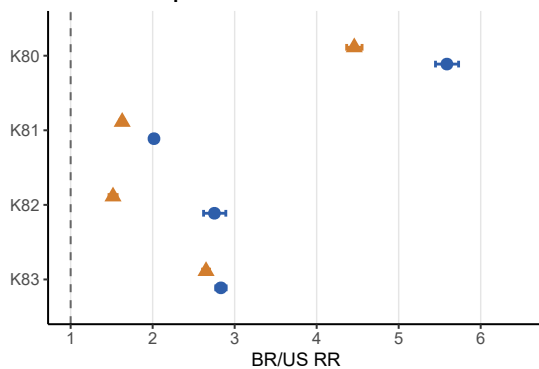
K80-K83 component BR/US RRs
