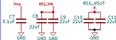
TPS63020 Decoupling Capacitors
