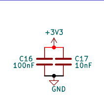
MCP2515 Decoupling Capacitors
