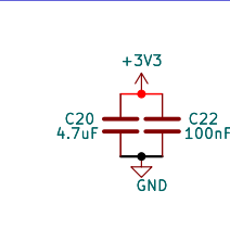
SN65HVD230 Decoupling Capacitors
