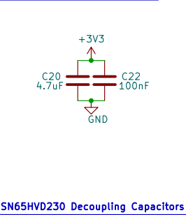
SN65HVD230 Decoupling Capacitors
