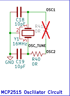
MCP2515 Oscillator Circuit
