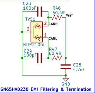
SN65HVD230 EMI Filtering & Termination
