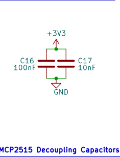
MCP2515 Decoupling Capacitors
