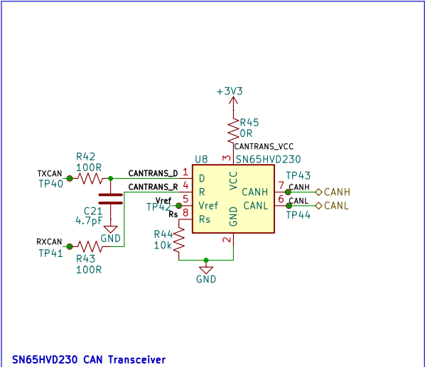
SN65HVD230 CAN Transceiver
