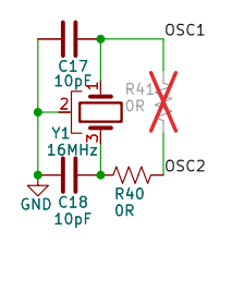
MCP2515 Oscillator Circuit
