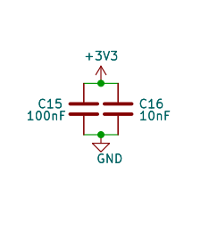
MCP2515 Decoupling Capacitors
