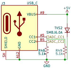
USB Connector
