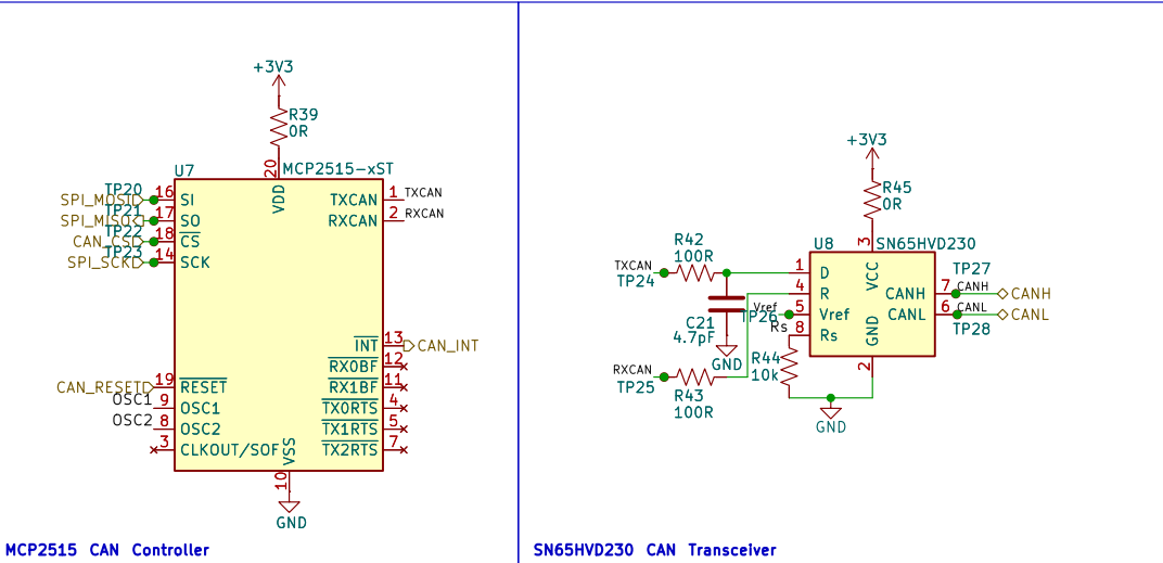
MCP2515 CAN Controller
