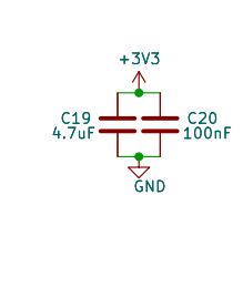
SN65HVD230 Decoupling Capacitors
