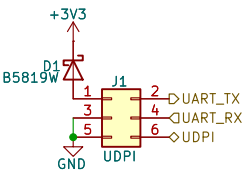
UPDI Connector
