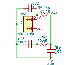
SN65HVD230 EMI Filtering & Termination
