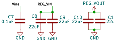
TPS63020 Decoupling Capacitor
