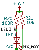
TPS63020 PG000D Pullup
