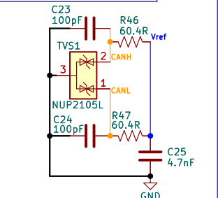
SN65HVD230 EMI Filtering & Termination
