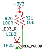
TPS63020 PGOOD Pullup
