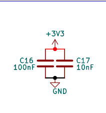
MCP2515 Decoupling Capacitors
