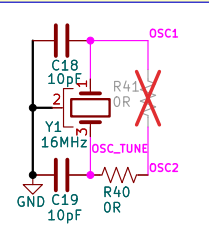
MCP2515 Oscillator Circuit
