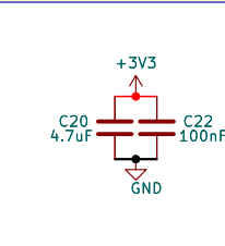
SN65HVD230 Decoupling Capacitors
