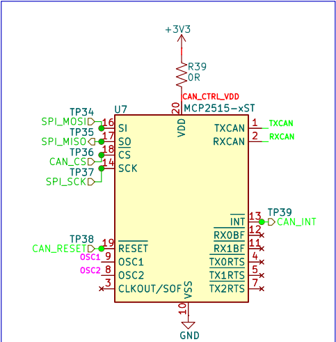
MCP2515 CAN Controller
