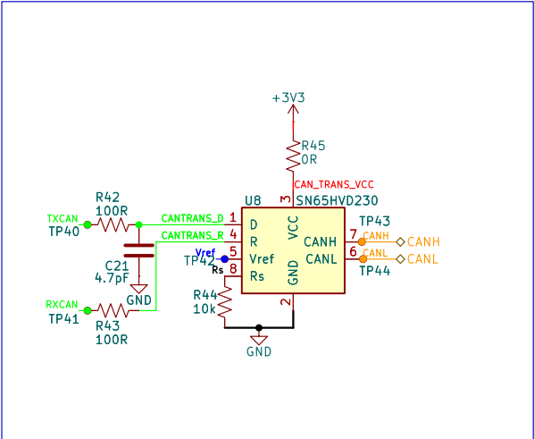
SN65HVD230 CAN Transceiver
