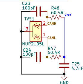
SN65HVD230 EMI Filtering & Termination
