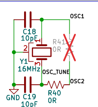
MCP2515 Oscillator Circuit
