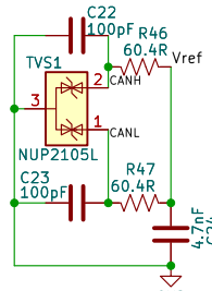
SN65HVD230 EMI Filtering & Termination
