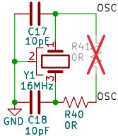
MCP2515 Oscillator Circuit
