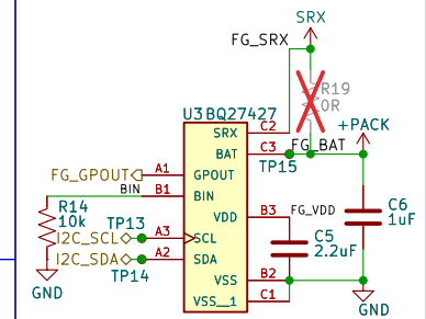
BQ27427 Fuel Gauge
