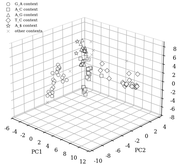
Figure 9: PCA projection of DNA-BERT hidden representations for the same 6-mer observed in different sequence contexts.
