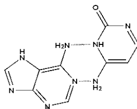
Figure 8: Mismatched Base Pair (AC)
