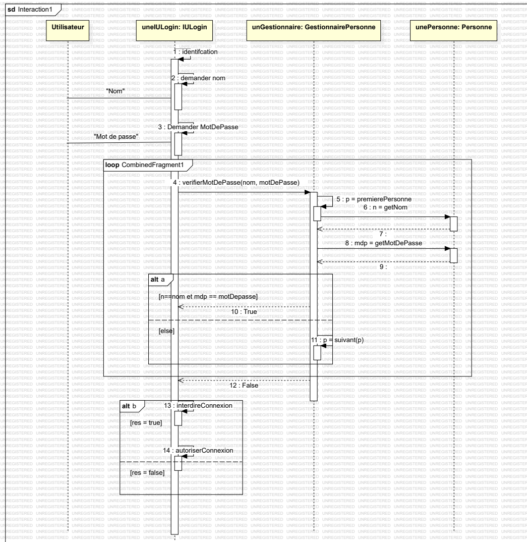
Figure 5: Sequence diagram describing the scenario of identifying a person to a system.
