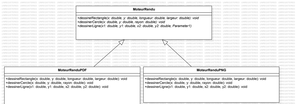
Figure 2: Class diagram for exporting geometric shapes
