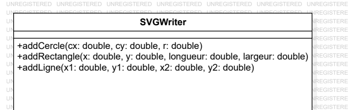
Figure 3: SVGWriter class from the external library
