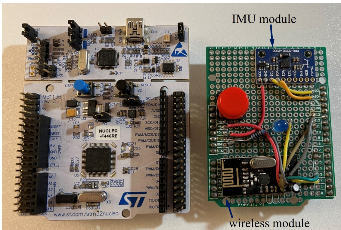
STM32 Nucleo dev board
