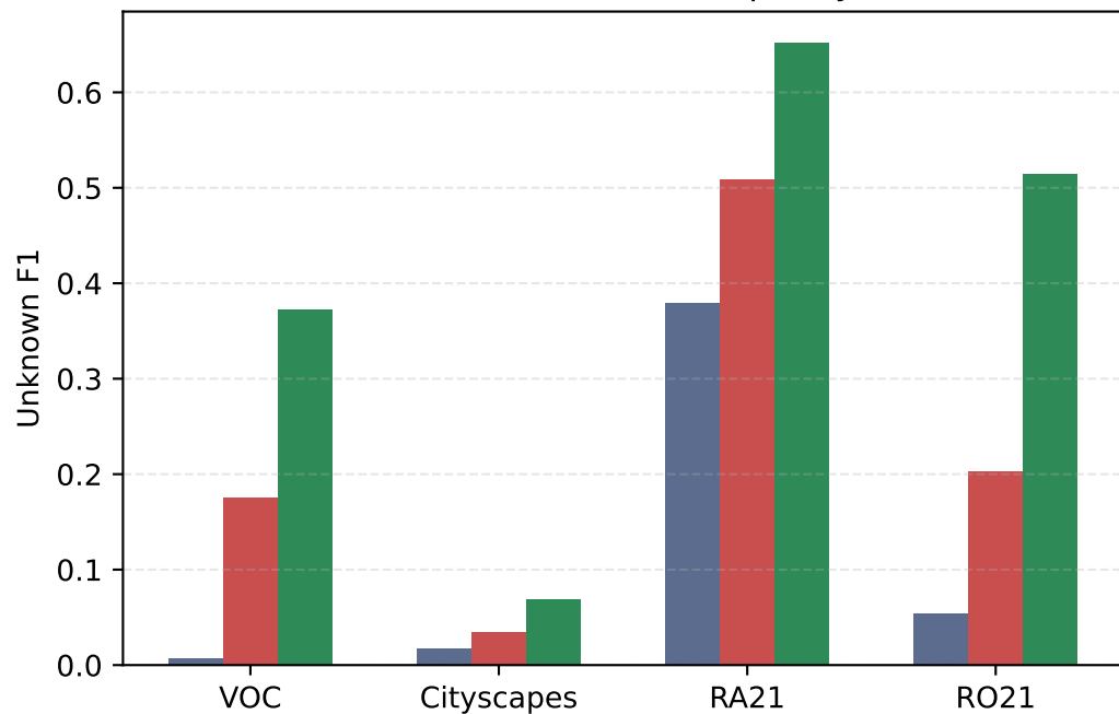
Unknown-structure quality
