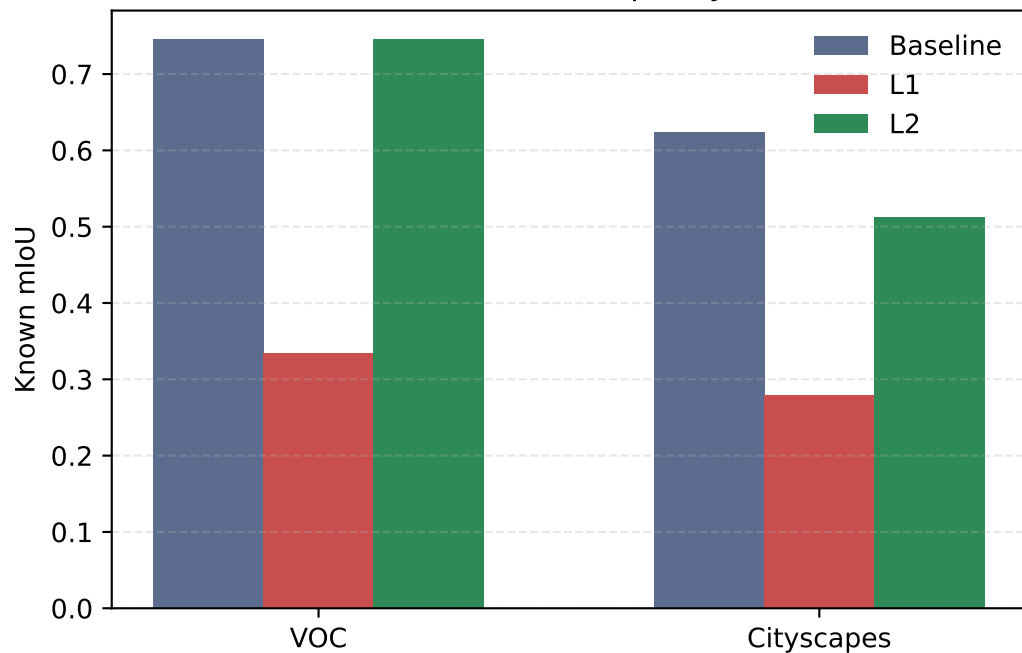
Known-class quality
