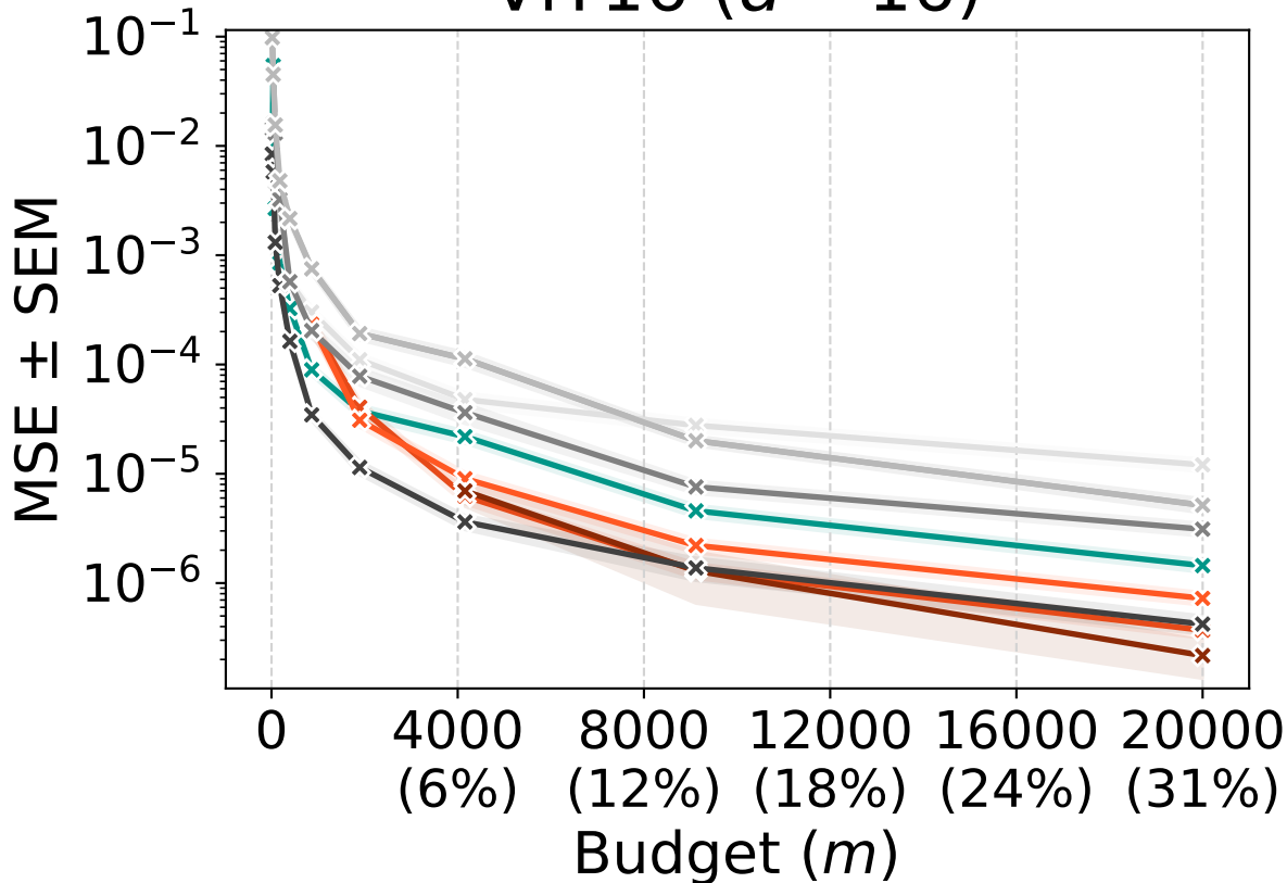
ViT16 ( d = 16 )
