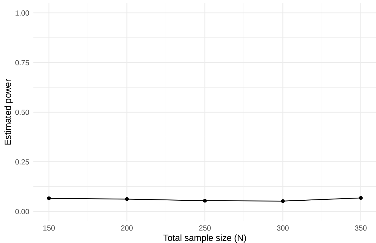
Monte Carlo power vs. total N for 3x3 mixed design
