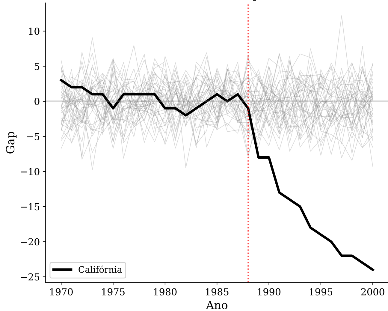
(a) Placebos in-space
