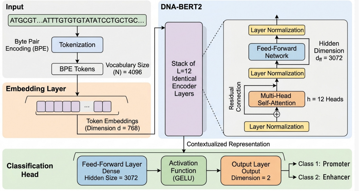
Figure 1: Architecture overview: DNA-BERT2 with a classification head.
