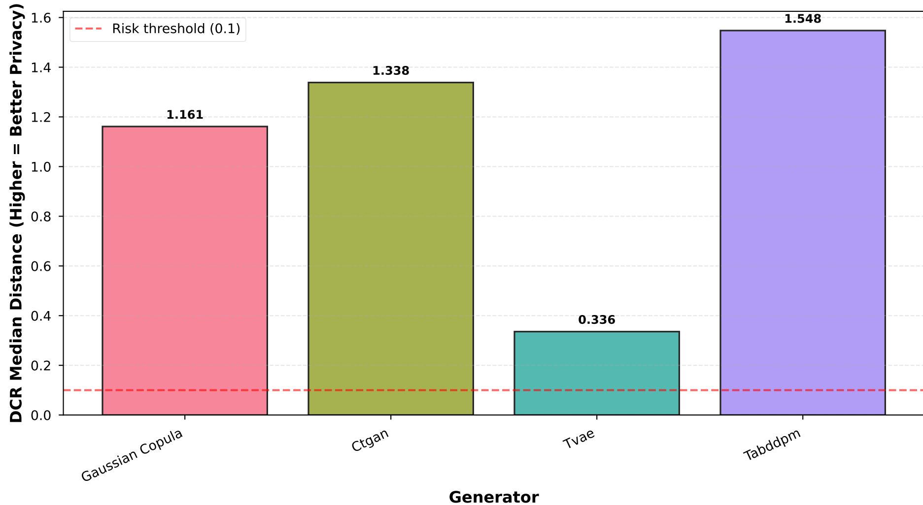
Privacy Risk Comparison - Sensitivity (1% DOE-noise)
