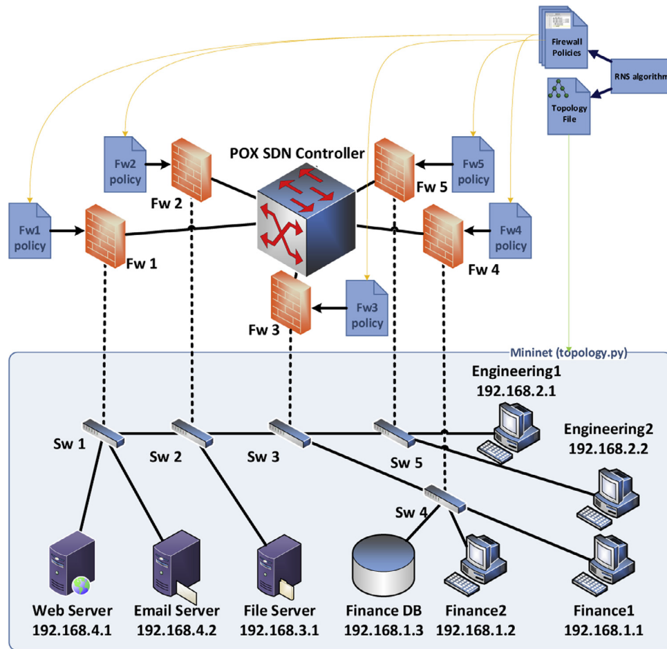
Fig. 12 – SDN simulation.
