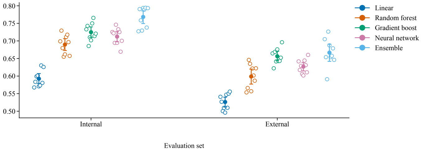
Balanced accuracy
