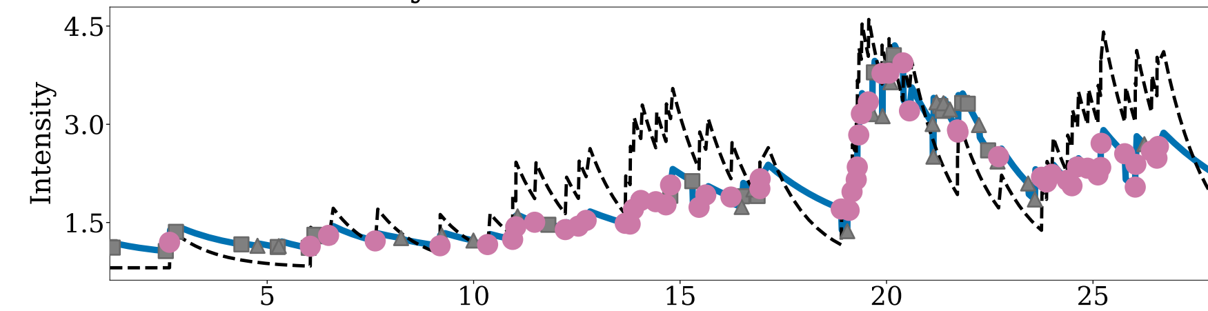
Synthetic 3D Hawkes Process
