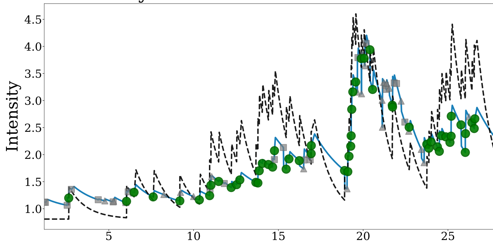
Synthetic 3D Hawkes Process
