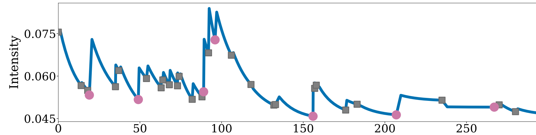
Retweet Dataset
