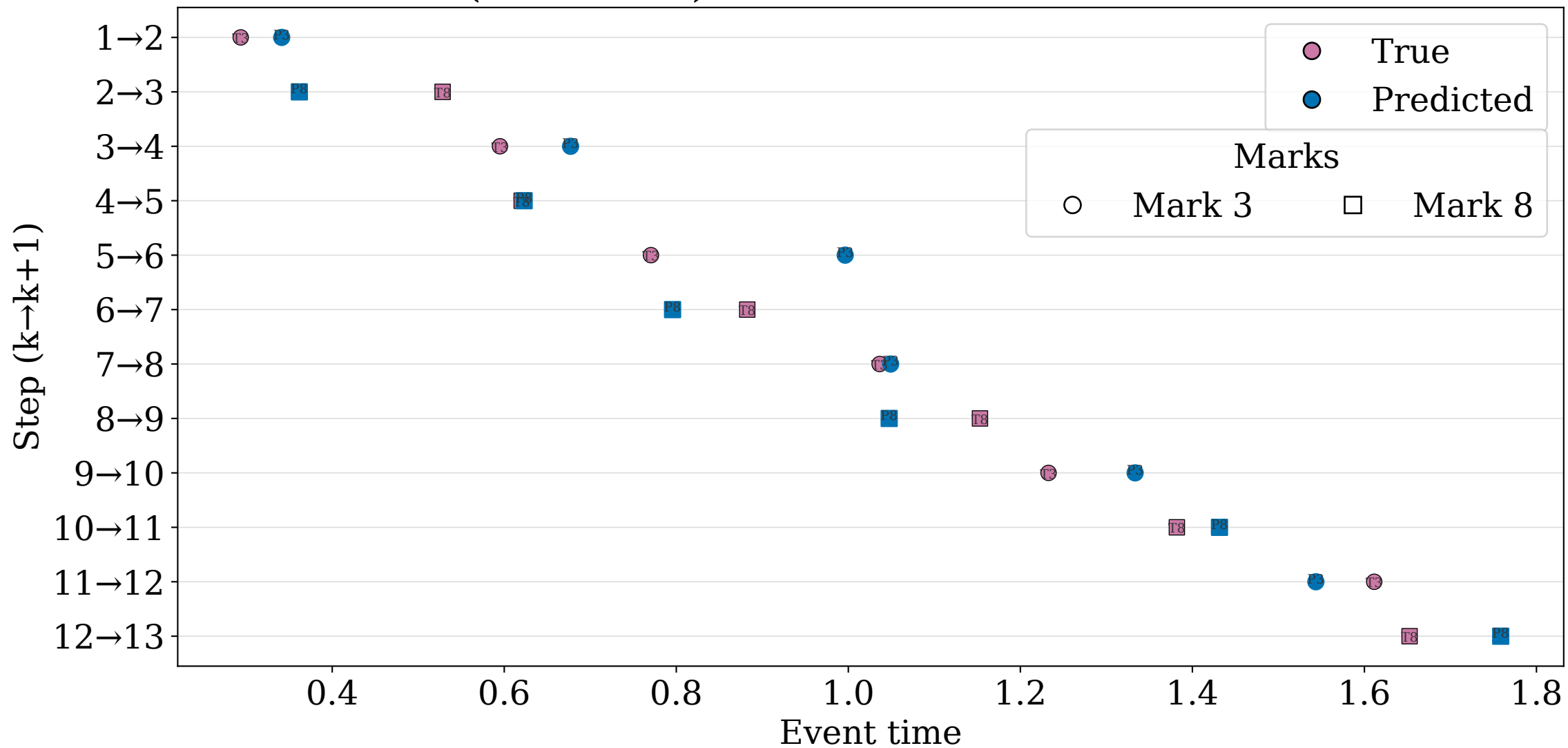
FIM-PP (fine-tuned) Taxi Dataset Next Event Prediction
