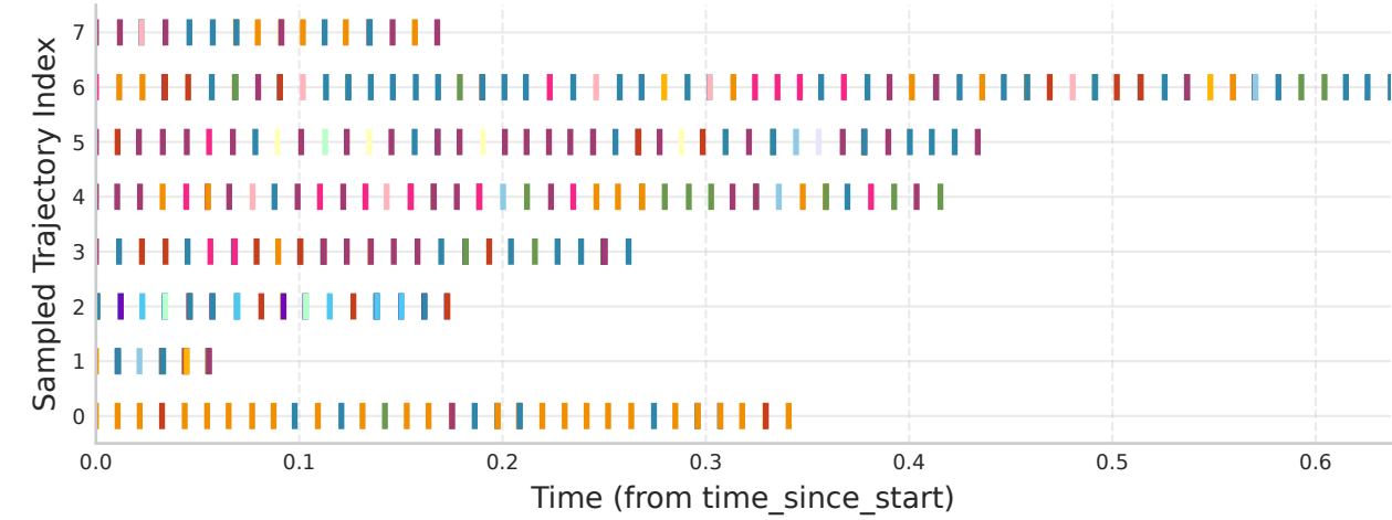
Raster Plot (8 Sampled Trajectories from train split)
