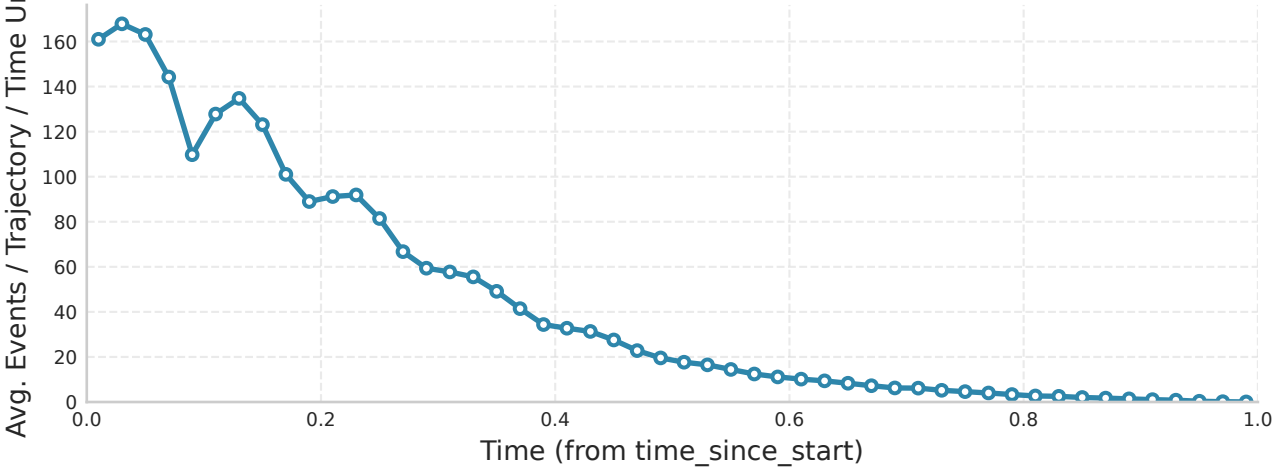
Aggregate Event Rate (train split)
