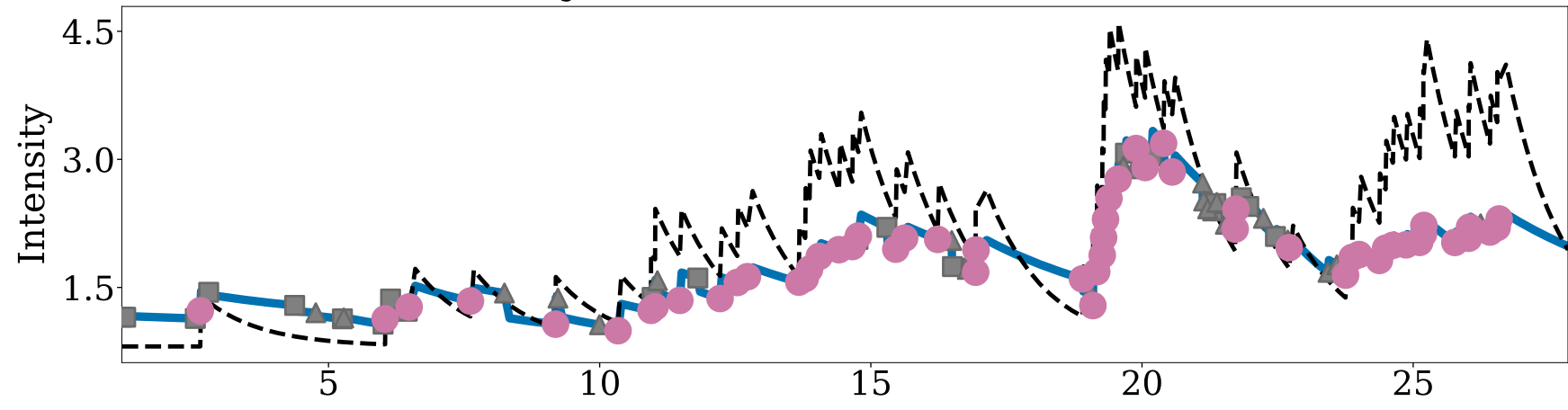
Synthetic Hawkes Process
