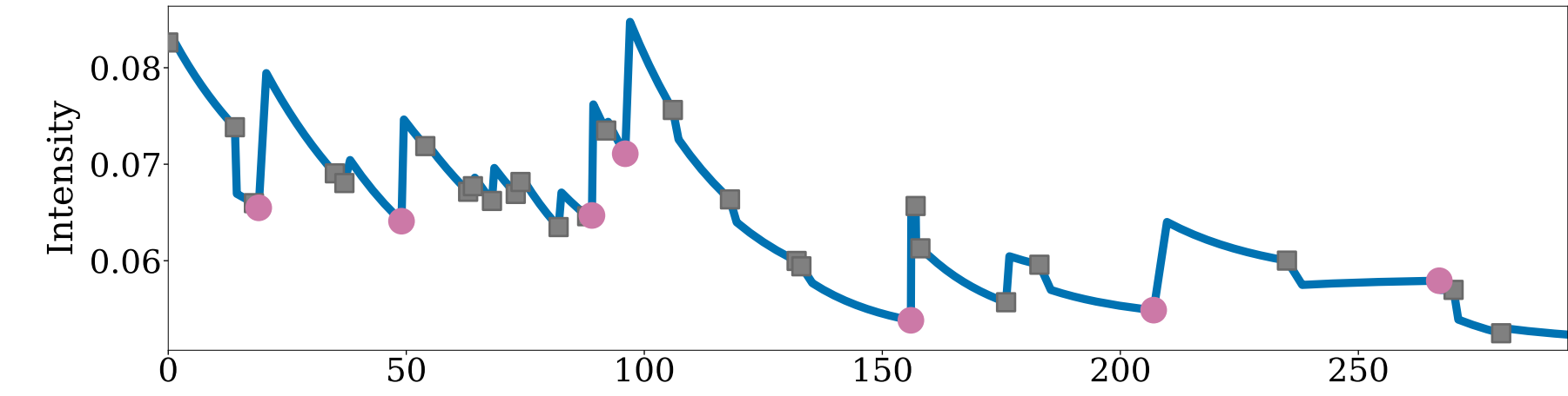
Retweet Dataset
