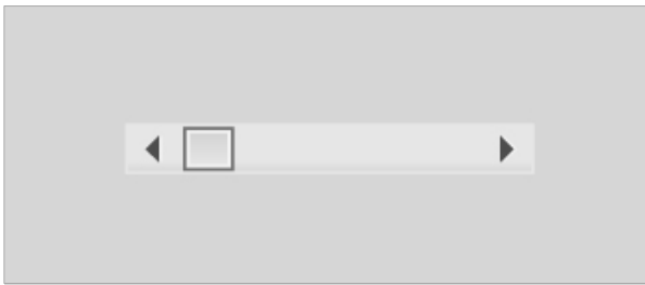
Figure 26: Unskinned ScrollBar.
