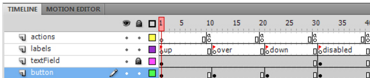
Figure 8: Button timeline.
