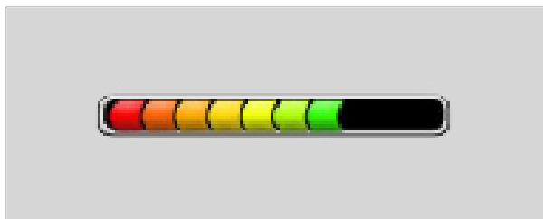
Figure 59: Skinned StatusIndicator.
