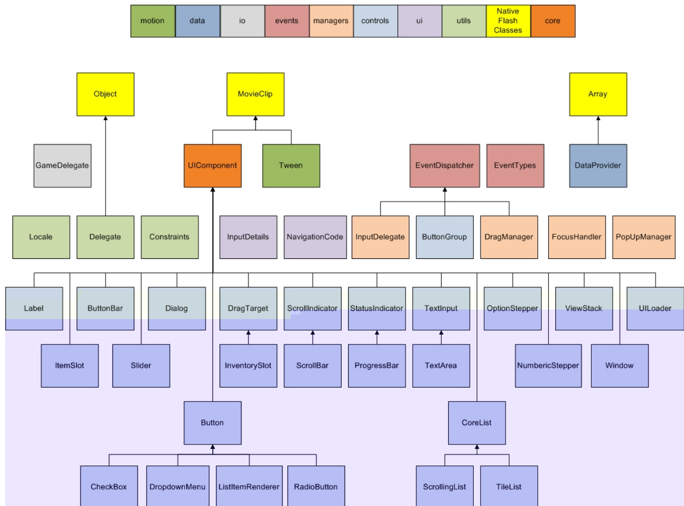
Figure 60: Scaleform CLIK class hierarchy.
