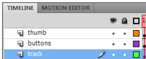
Figure 27: ScrollBar timeline.
