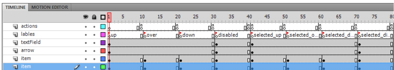
Figure 44: DropdownMenu timeline.
