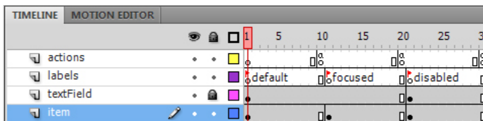
Figure 15: TextInput timeline.
