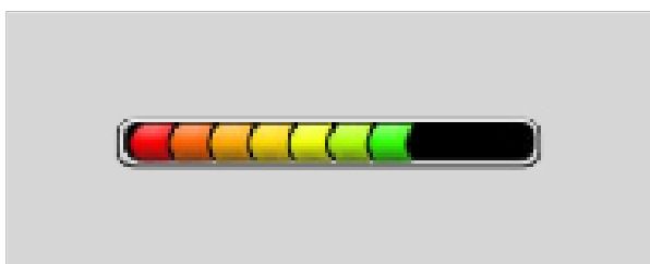
Figure 57: Skinned StatusIndicator.
