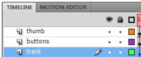
Figure 27: ScrollBar timeline.
