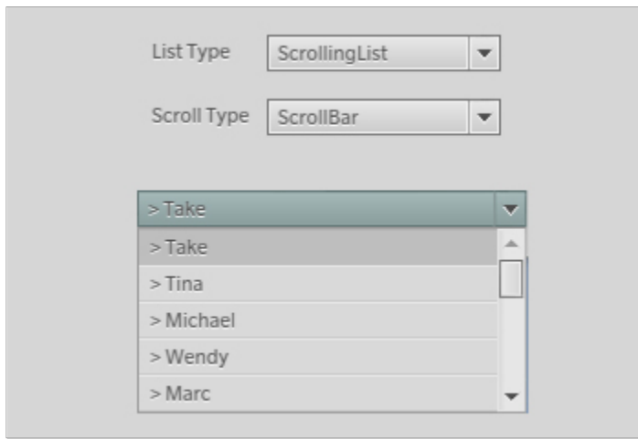
Figure 43: Unskinned DropdownMenu.
