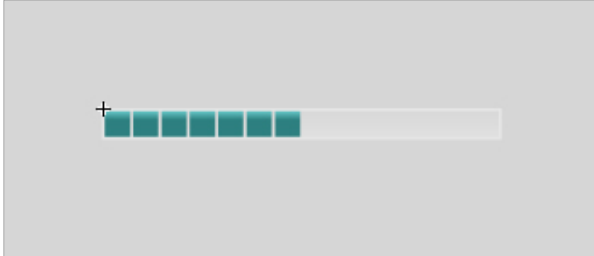
Figure 53: Unskinned StatusIndicator.
