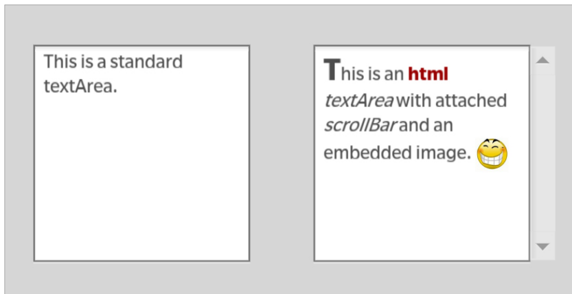
Figure 16: Unskinned TextArea.
