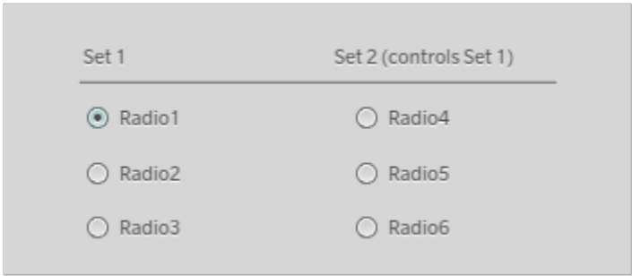
21: ButtonGroup.
