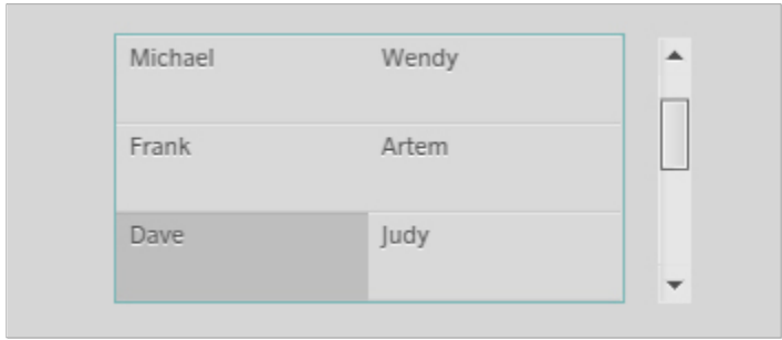
41: TileList.
