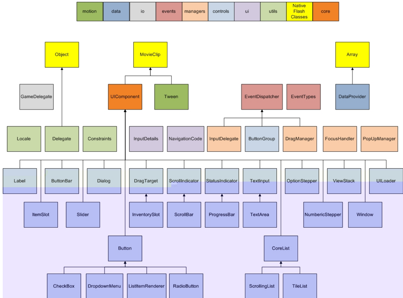
60: Scaleform CLIK
