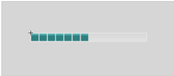
55: StatusIndicator.
